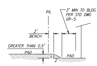
TYPICAL REAR LOT GRADING DETAIL N.T.S.
